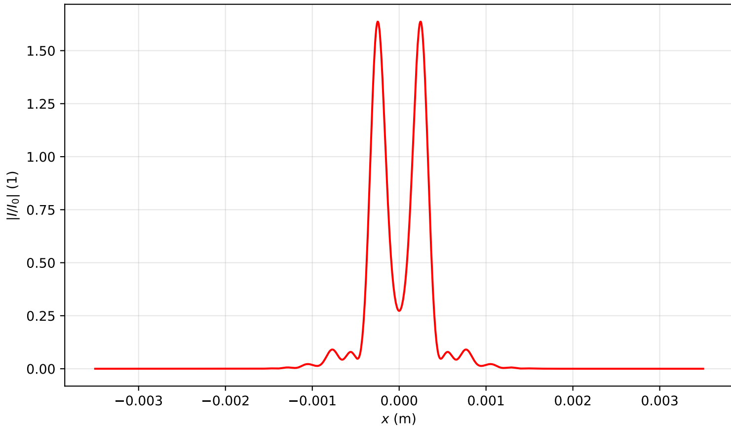
Intensity profile I(x, y = 0, z = 1.194)/I_0 , P_{in}=2.5P_{cr} , artificial time
